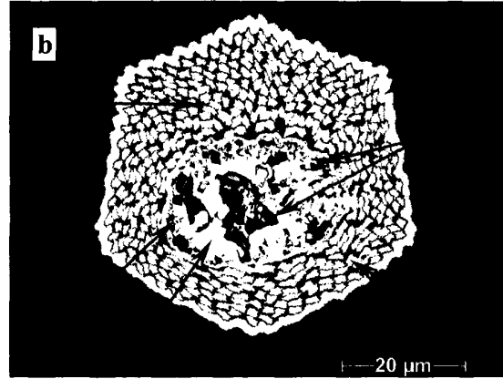
Fig. 1. SEM-BE images of the wire (a) and bundle (b) cross-sections prior to heat treatment. Mg-Cu-Sn ternary particles were seen in the core prior to any heat treatment. The voids are most likely a polishing artifact.
