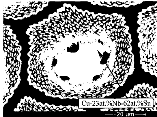
Fig. 2. SEM-BE image of a Cu-Nb-Sn ternary phase growing into the core region after a heat treatment of 150h/362°C. A similar structure surrounds the inner core of filaments.
