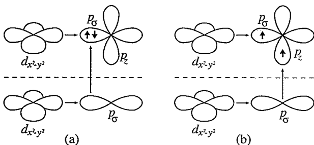
FIG. 5. Schematic illustration of superexchange processes giving rise to antiferromagnetic and ferromagnetic interplanar interactions. A hole hops from the d_{x^2-y^2} orbital of a Cu atom to the p_\sigma orbital of a neighboring O. (a) An interplanar hop between two O's which takes place into a p_\sigma orbital gives rise to an antiferromagnetic coupling. (b) It is about 4 times more probable that an interplanar hop ends up into a p_z orbital which extends far below and above the O site. This process gives rise to ferromagnetic coupling. The third interaction mechanism arises from direct ferromagnetic exchange between one hole remaining at the d_{x^2-y^2} orbital and another entering a neighboring p orbital by an interplanar hop.
